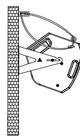
HORIZONTAL WALL-MOUNT UB-L + SC-15
