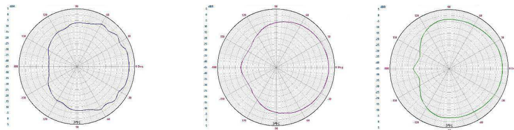
Fig. 6. Back energy rejection at 40 Hz / 50 Hz / 63 Hz
