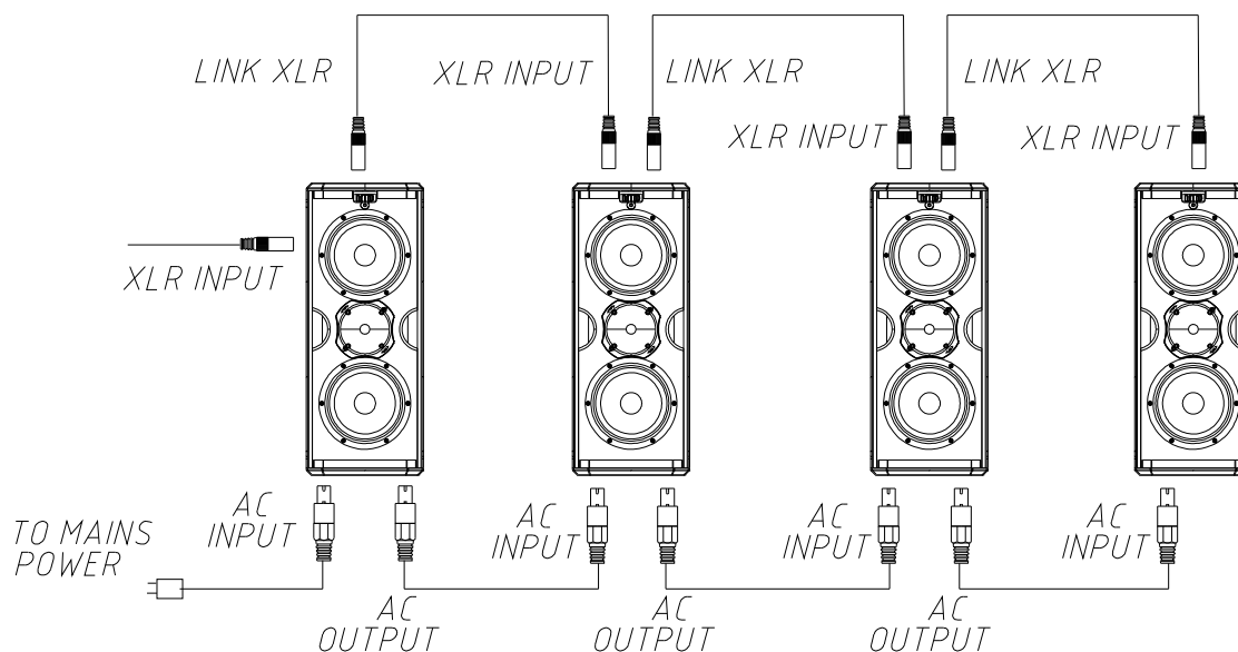
Fig. 3. Parallel connection for S26 (signal and mains)
