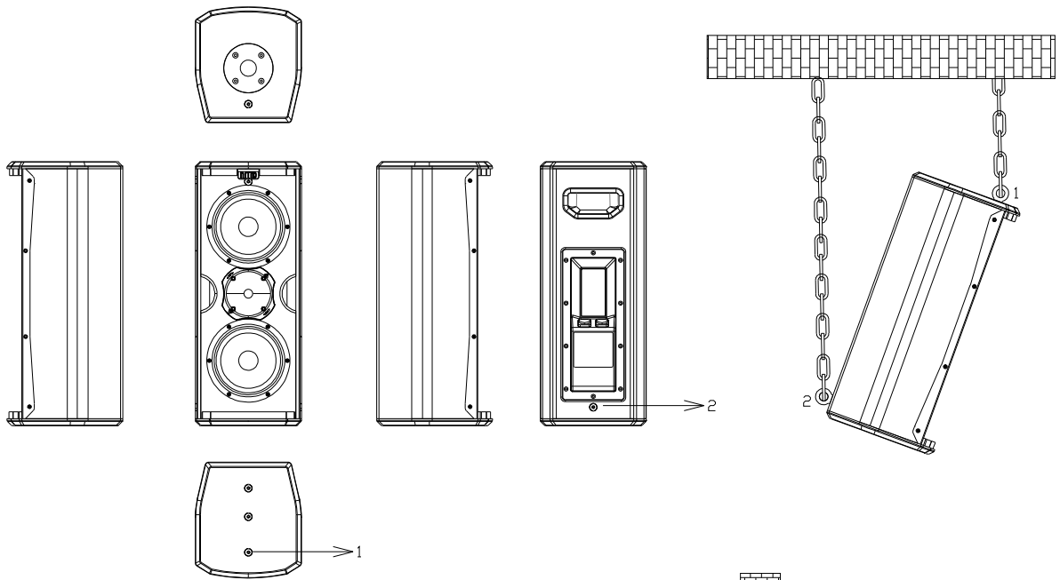
Fig. 9. S26 rigging points
